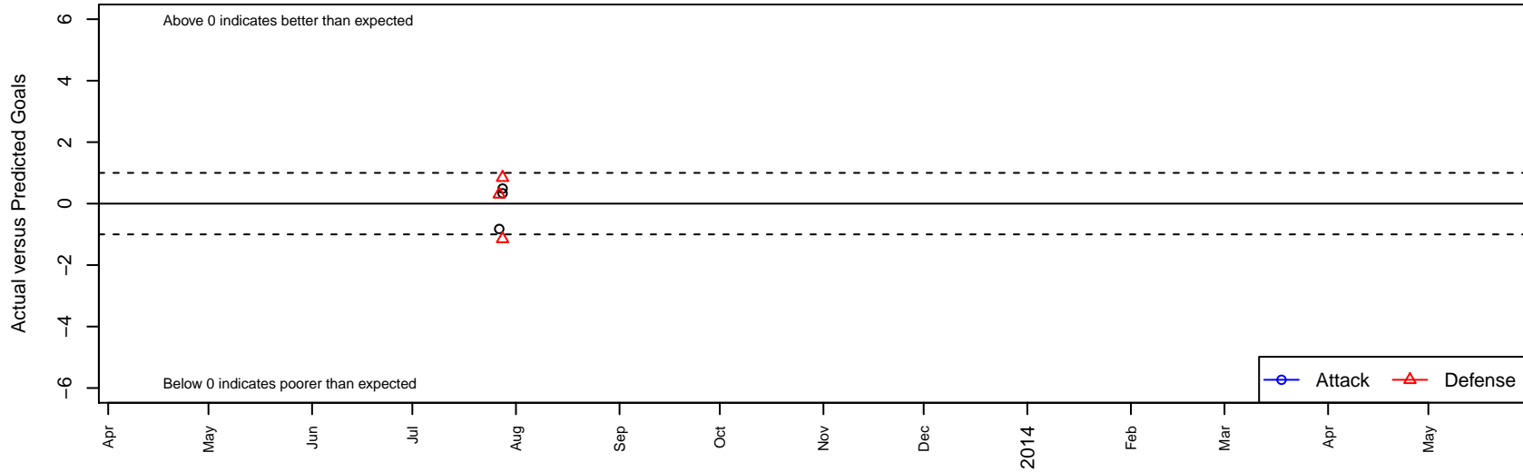
DFW Tejanos 98 Premier B97 Dots are actual minus expected GF (blue circles) and GA (red triangles). Blue line is smoothed change in attack strength. Red is smoothed change in defense strength.
